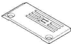
ART. 9094/1 - # 14-806 (1/8") ART. 9094/2 - # 14-807 (5/32") ART. 9094/3 - # 14-808 (3/16") ART. 9094/4 - # 14-809 (7/32") ART. 9094/5 - # 14-810 (1/4")
